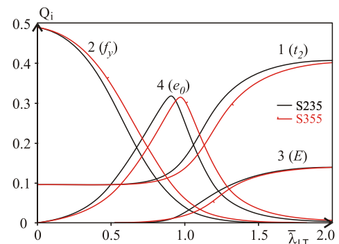
Fig. 8. First order quantile contrast indices for M = 4 .
