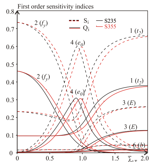
Fig. 4. First order sensitivity indices S_i , Q_i for M = 8 .
