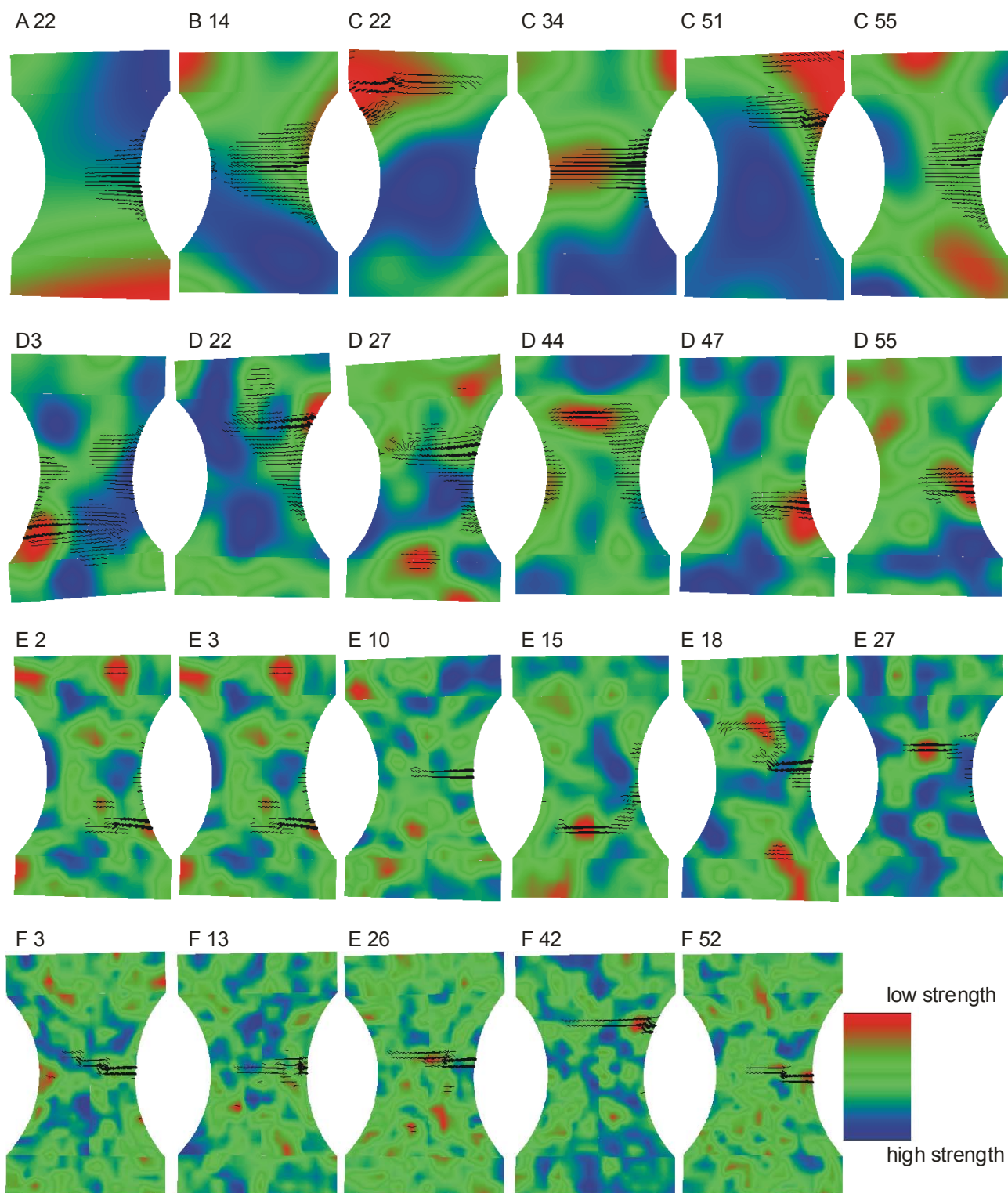
Figure 4. Simulated random strength field realizations and corresponding crack patterns in deformed specimens. Field simulated and crack widths computed in integration points.
