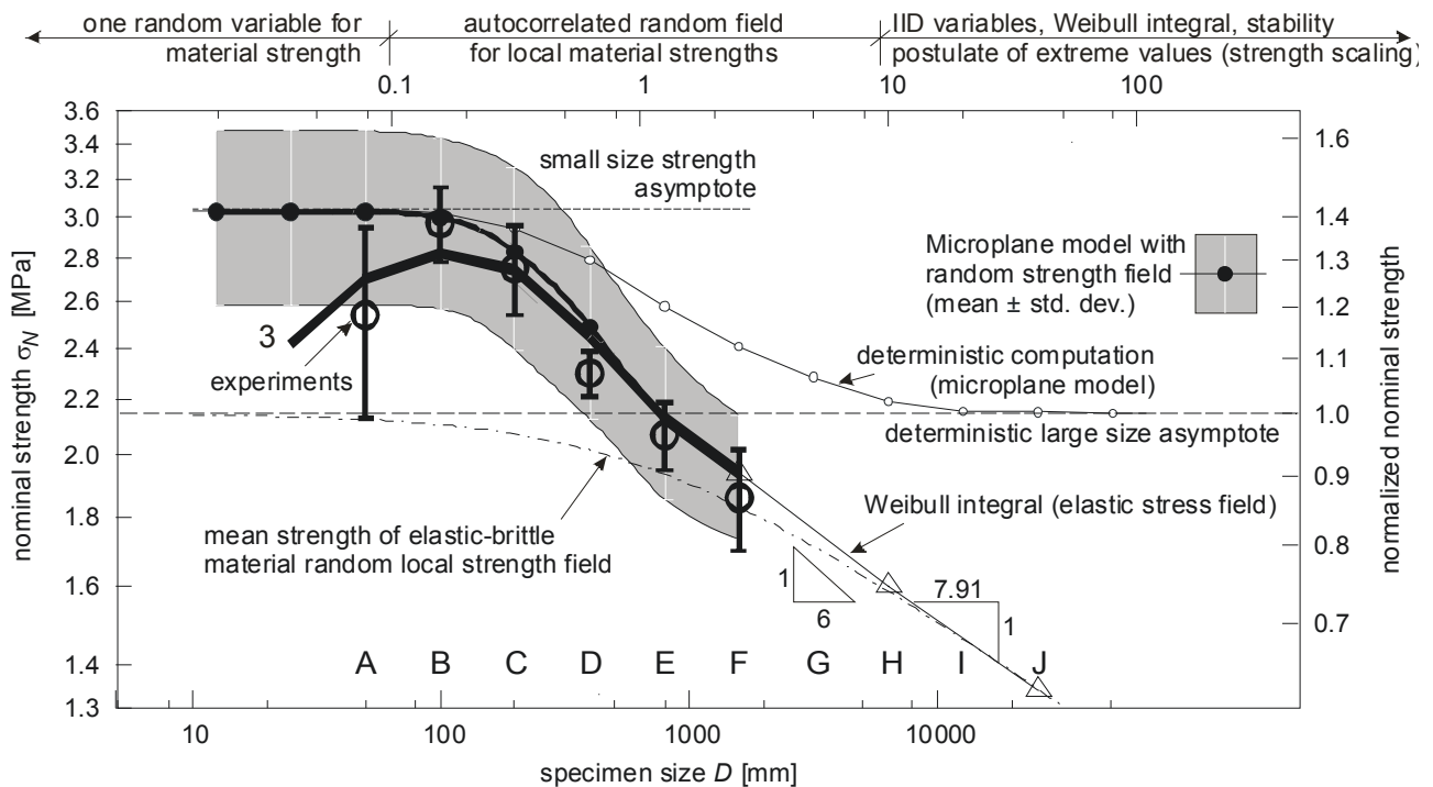
Figure 6. Comparison of results in size effect plot.
